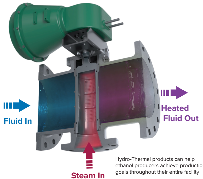
Hydro-Thermal Solaris Heater
